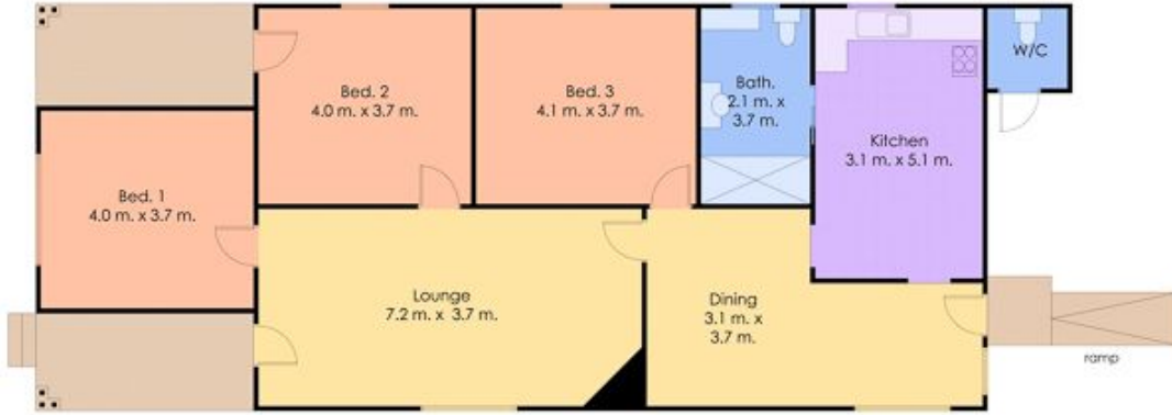
Floor Plan Total Internal Floor Area: 118 sqm
