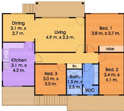
Upper Floor Plan Total Internal Floor Area: 170 sqm
