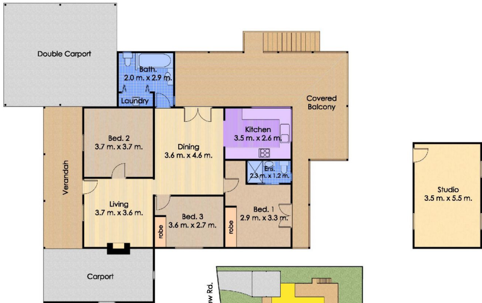
Floor Plan Total Internal Floor Area inc. Studio: 108 sqm
