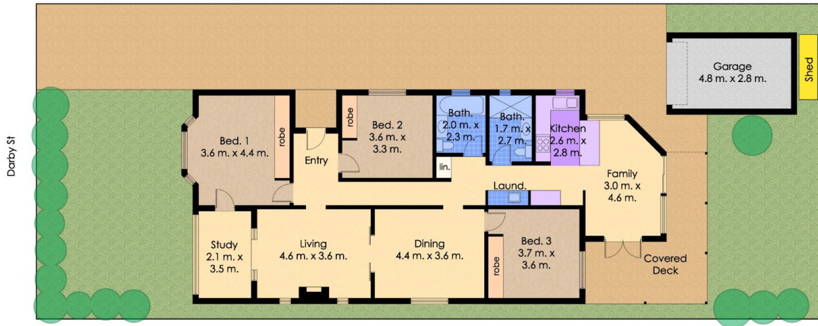
Floor Plan Total Approx. Internal Floor Area: 144 sqm
